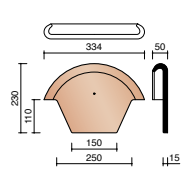
P000 1240 ☉ Fronton 230 mm
